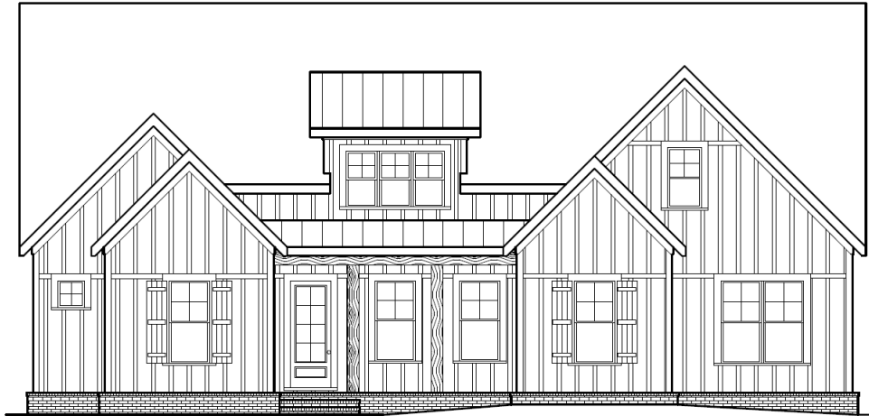
ELEVATION "A"
