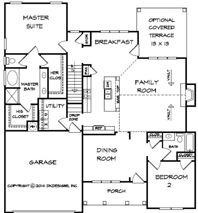
MAIN LEVEL FLOOR PLAN - A
